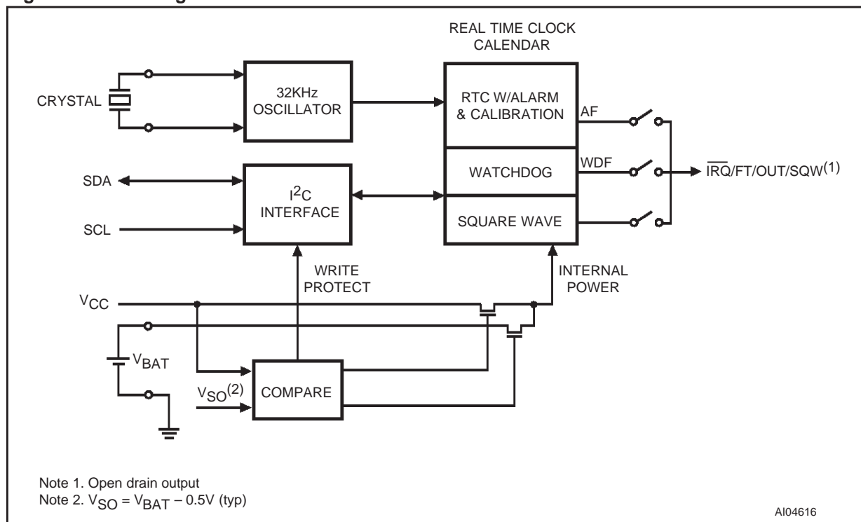
Figure 6. Block Diagram
